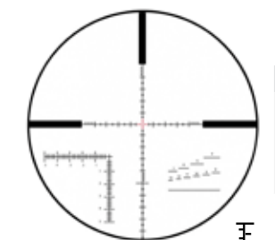
MSR 2 RETICLE SUBTENSION
