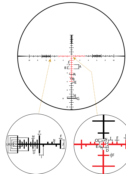
SCR MOA RETICLE SUBTENSION
