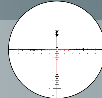
SCR™ / SCR™-MOA Reticle
