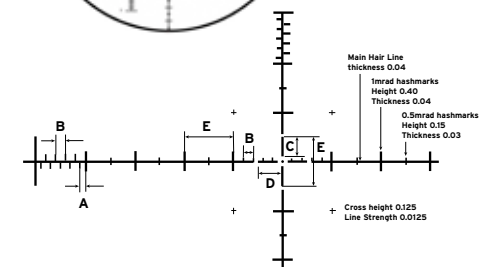
C2 RETICLE SUBTENSION
