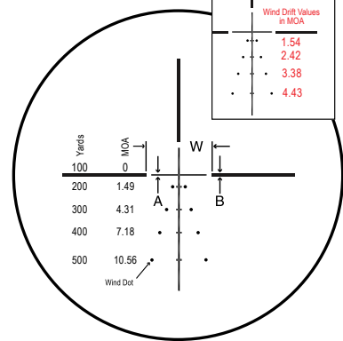
PLEX S1 LOW MAG
