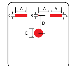
C2 RETICLE SUBTENSION
