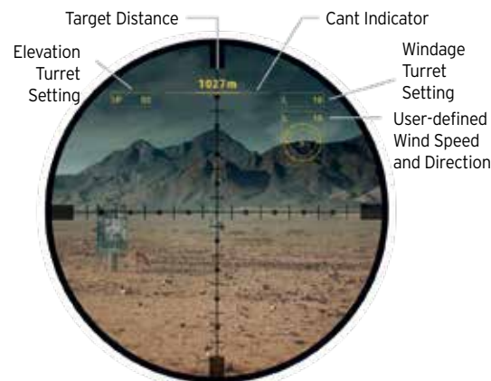
Customized Display A sophisticated user Interface presents the precise firing solution in your field of view.
